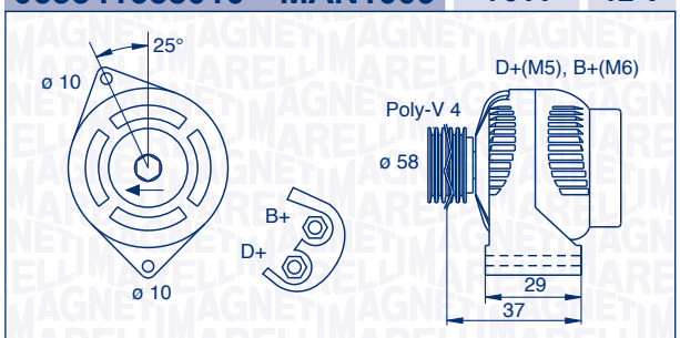
063341658010 – MAN1009 75 A 12 V
