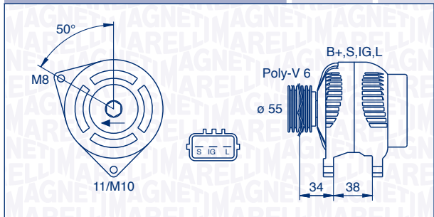
063377432010 – MAN7432 90 A 12 V
